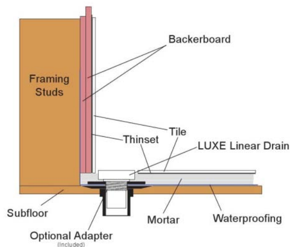
Wall Cross-Section Installation
